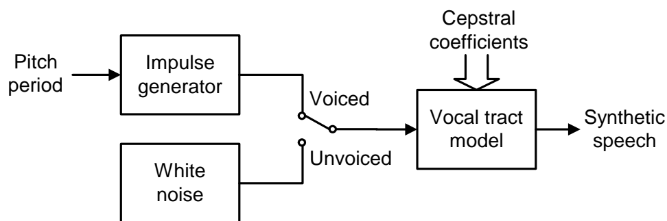
Fig 1. Parametric cepstral speech model.
