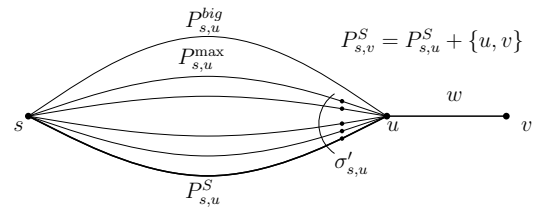
Figure 4: An extension of \delta(s, u) -almost shortest path by an edge contained in a shortest path
