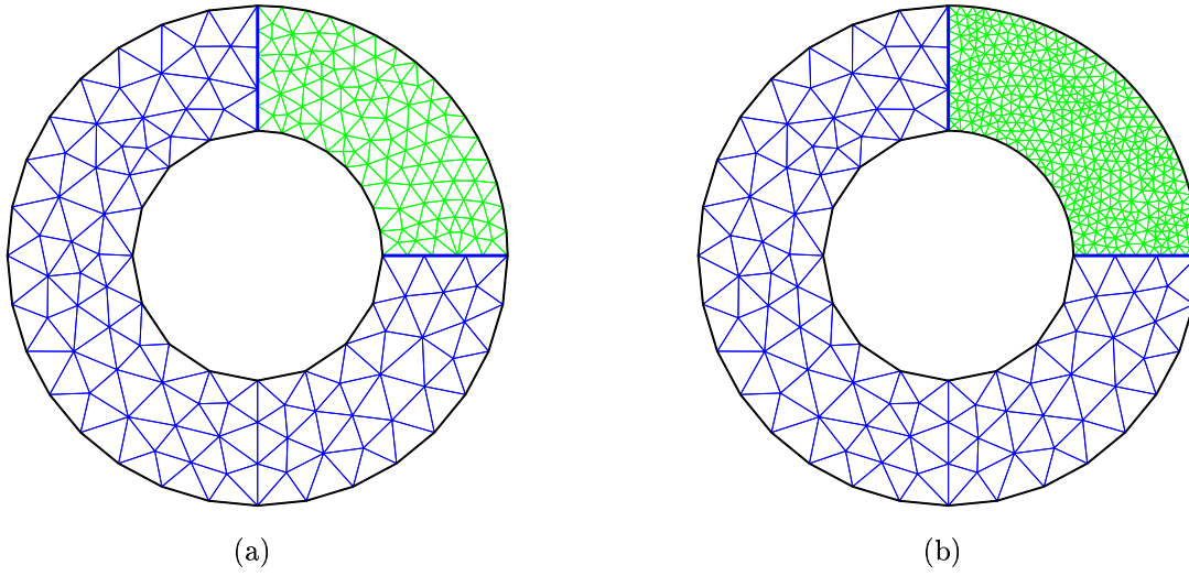
Figure 12: Partition of \Omega and two versions of the appropriate mesh for problem (5.2).
