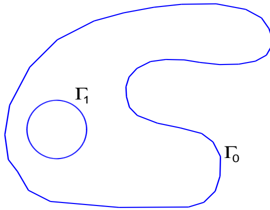
Figure 8: Computational domain \Omega for problem (5.1).
