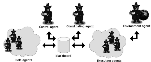
Figure 1: The architecture of the MAS simulating enhanced processes.
