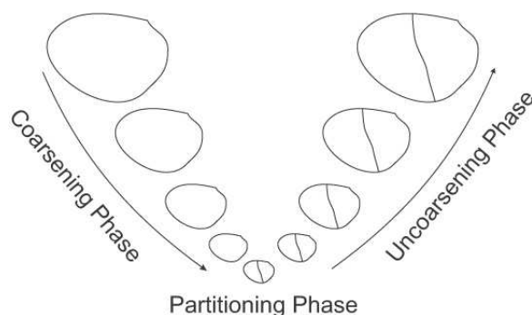
Figure 1: Multilevel bisection
