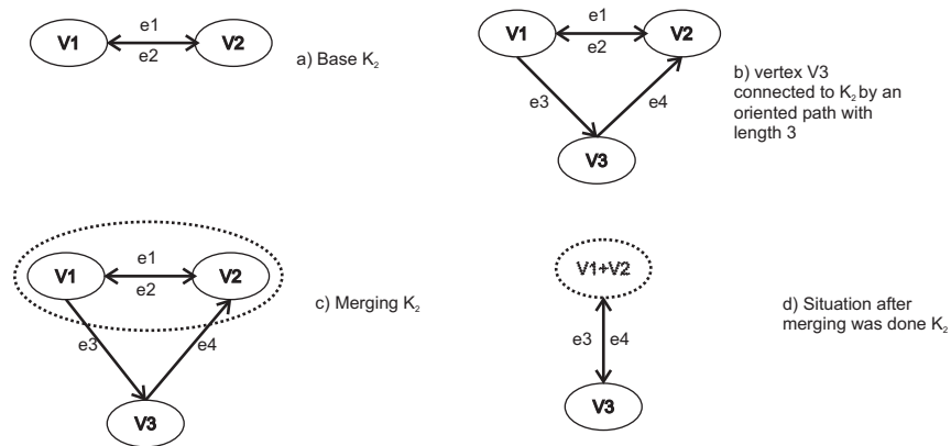
Figure 3: G2H algorithm for transforming edges into nets
