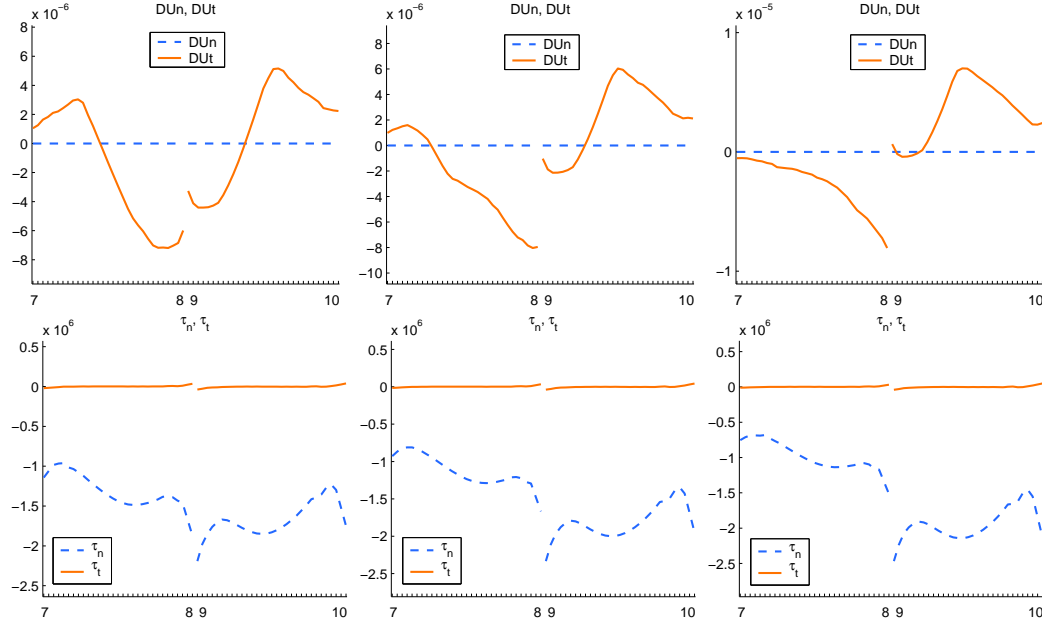
Fig. 4. Normal and tangential components of the displacement and of the stress vectors on the contact boundary in the area of both condyles for MODEL I, II, III characterizes mutual shift of the contralateral points of both components of the knee joint in the tangential direction. The analysis of the tangential component of the displacement vector points a relatively small shifts in both condylar components of the joint. The character of their process is a little different for the studied axial deviation. From the values of both components of the displacement vector we get then real mutual shift of the contralateral points of the contact in the space. Normal and tangential stresses on the contact in both condylar parts of the knee joint characterizes loading relations on the both condylar parts of the knee joint. We see that on the contact between both femorotibial parts of the knee joint the pressure is observed in both condyles.
