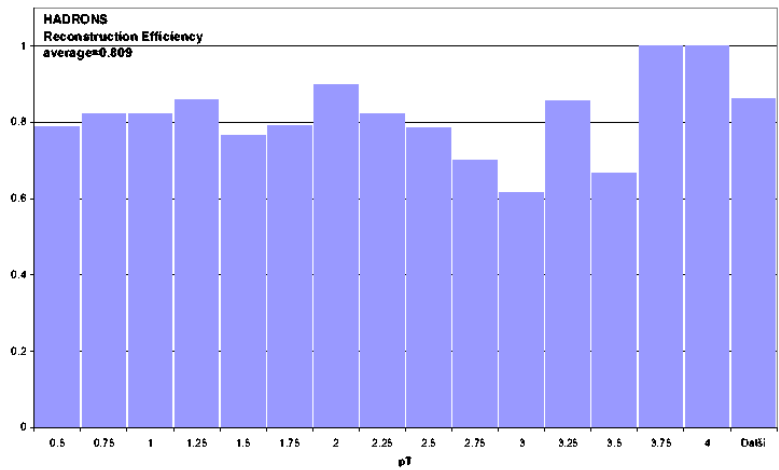
Fig. 3. Reconstruction Efficiency as function of pT, hadrons
