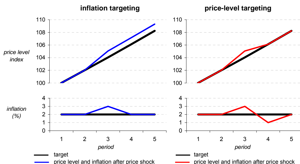
Figure 1: Illustration of Price-Level and Inflation Paths under Inflation Targeting and under Price-Level Targeting
