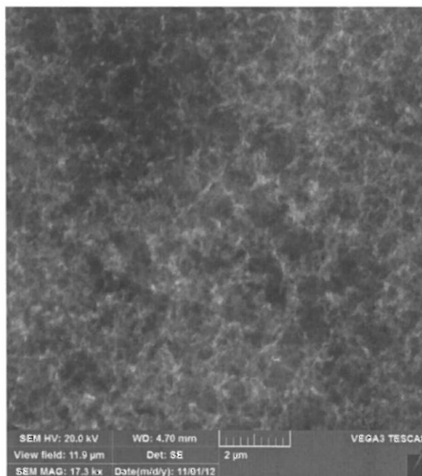
Figure 1. SEM image of NP's generated by evaporation/condensation of metallic Pb at T_R=860 °C, Q_R=1000 cm 3 /min.
