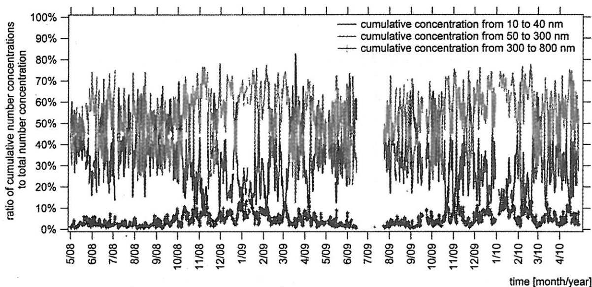
Fig. 2 Cumulative concentrations for particles smaller than 40 nm, between 50 nm and 300 nm, and particles larger than 300 nm in diameter, compared to the total particle number concentrations. The hourly means were replaced with daily medians for a better readability.
