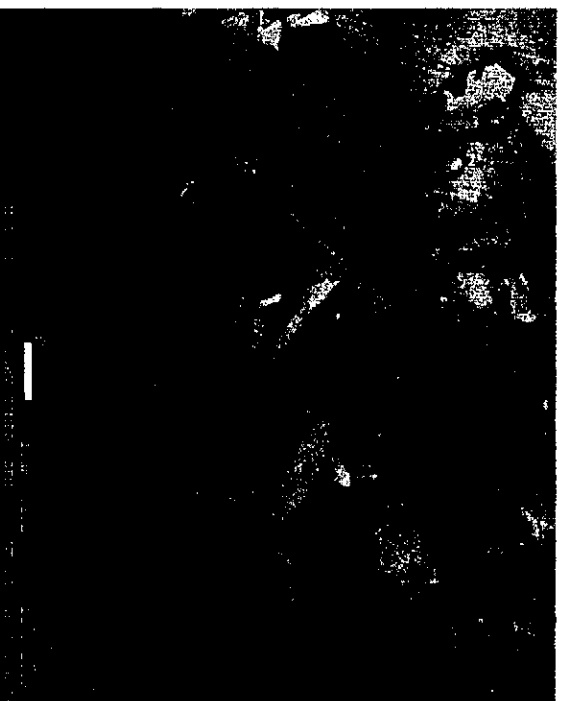
\text{Cu}_3(\text{Ge}_{0.5}\text{Si}_{0.5}) nanodesičky
